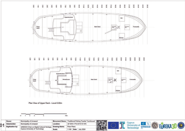
Figure 31. Plan View
