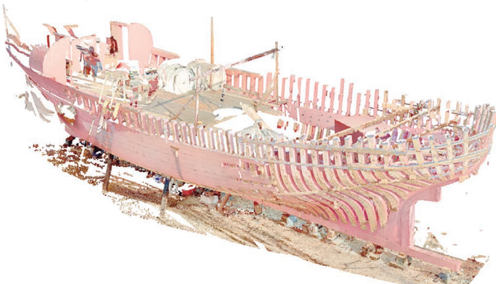
Figure 23. TLS Point Cloud result
