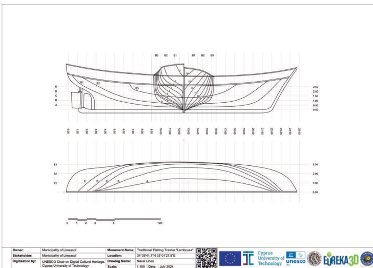
Figure 30. Naval Lines
